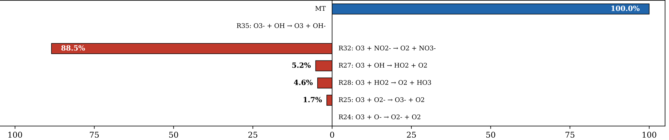
(c) NO 2 - (Σsrc = 1.80e-08 M/s)
